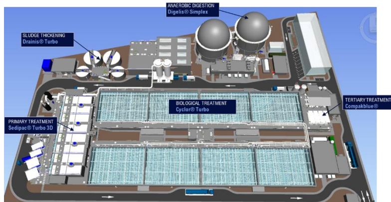
3D design of Central Manila Sewerage System project that will leverage SUEZ's pioneering technologies.
